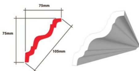
BR 6 XPS 75 x 75 x 105mm
