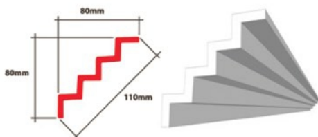
BR 3 XPS 85 x 85 x 115mm
