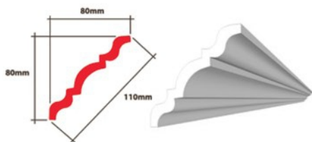
BR 2 XPS 80 x 80 x 110mm
