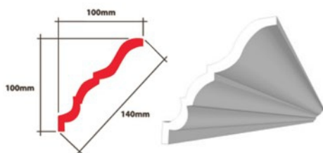
BR 9 XPS 100 x 100 x 140mm
