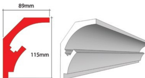
CORNICE 003 XPS 115 x 89 x 145mm
