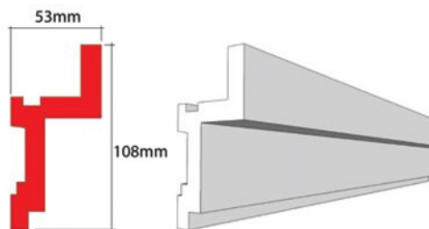
CORNICE 001 XPS 108 x 53 x 120mm
