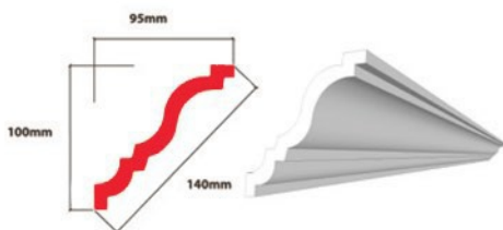
ALINA 100 x 95 x 140mm
