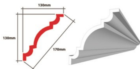
BR 11 XPS 130 x 130 x 170mm
