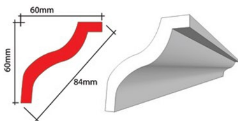
BR 12 XPS 60 x 60 x 85mm
