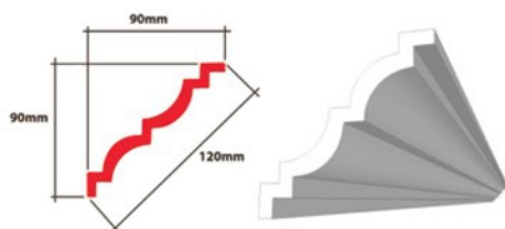
BR 4 XPS 90 x 90 x 120mm
