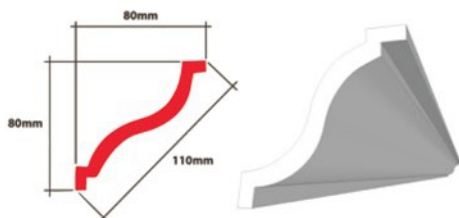
BR 8 XPS 80 x 80 x 110mm
