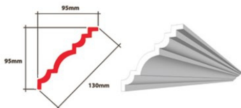
BR 1 XPS 95 x 95 x 130mm
