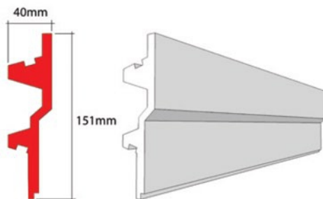
CORNICE 002 XPS 151 x 40mm
