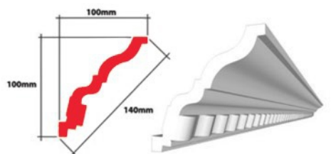
JULIET EPS 100 x 100 x 140mm
