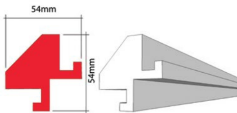
CORNICE 004 XPS 54 x 54 x 55mm
