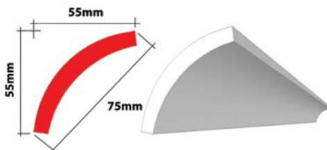
BR 13 XPS 55 x 55 x 75mm
