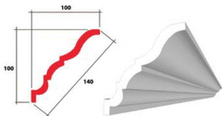
TROY 100 x 100 x 140mm
